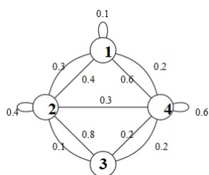
Fig. 6.2 Sample graph
